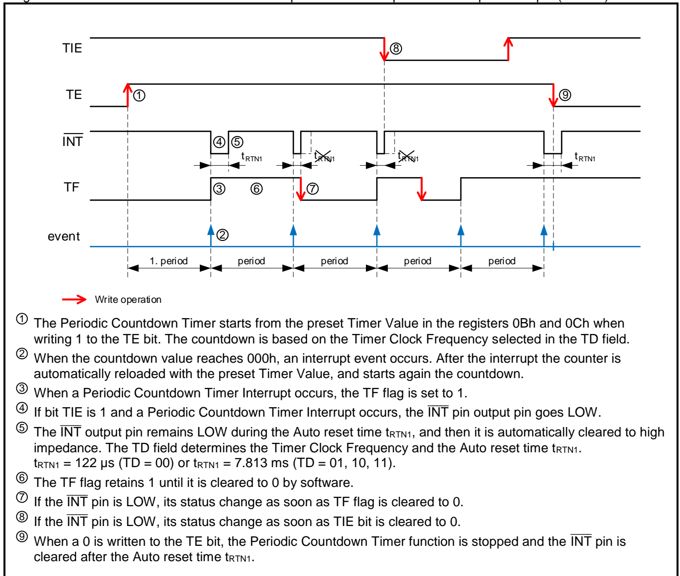
Diagram of the Periodic Countdown Timer Interrupt function: Example with interrupt on \overline{\text{INT}} pin (TIE = 1).
