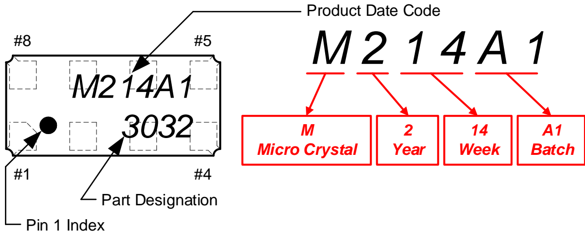
Laser marking RV-3032-C7 Package: (top view)
