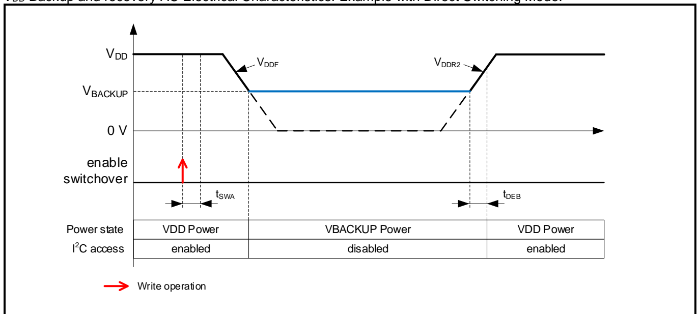
V_{DD} Backup and recovery AC Electrical Characteristics: Example with Direct Switching Mode.
