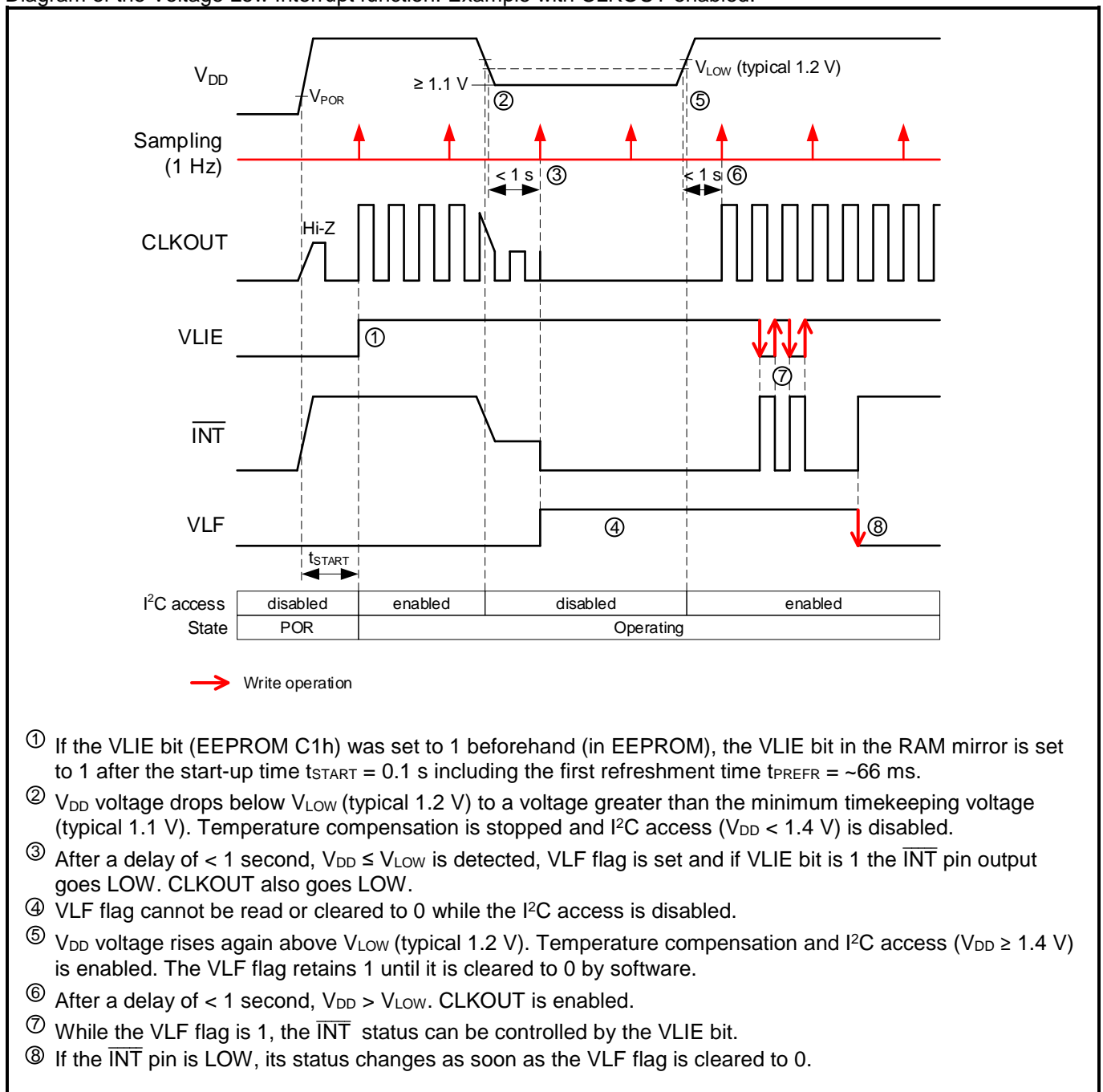
Diagram of the Voltage Low Interrupt function: Example with CLKOUT enabled.
