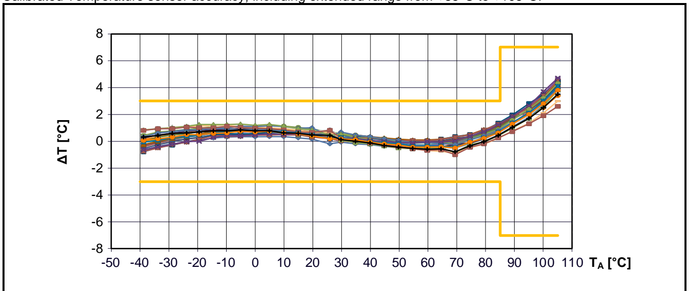
Calibrated Temperature sensor accuracy, including extended range from +85°C to +105°C:
