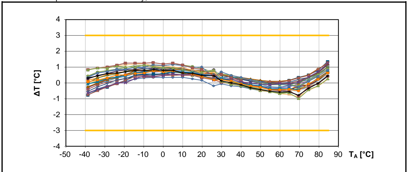
Calibrated Temperature sensor accuracy, T A = -40°C to +85°C:
