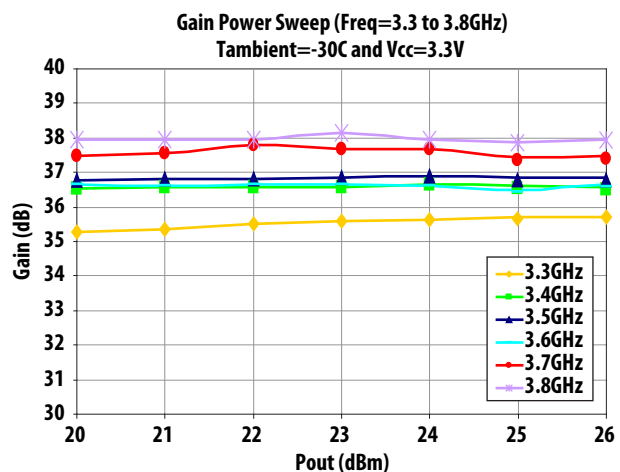
Figure 10. Gain Power Sweep at Vcc=3.3V and -30C over Frequency
