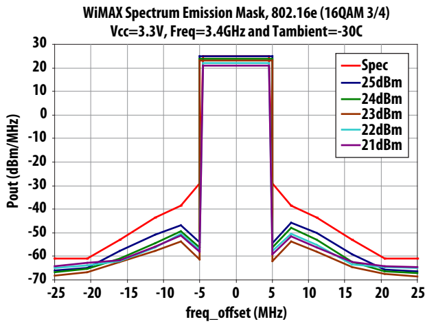
Figure 33. SEM at Vcc=3.3V, -30C and 3.4GHz over Vcc (2dB Post-PA loss assumed)
