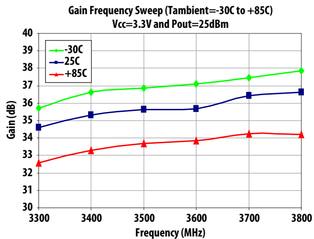
Figure 8. Gain Frequency Sweep at Vcc=3.3V and Pout=25dBm over Tambient
