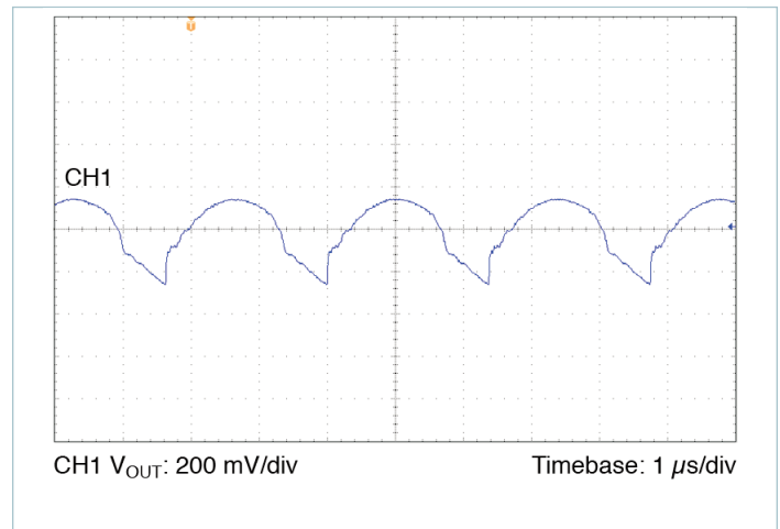
Figure 19 — Output voltage ripple, V_{IN} = 24\text{ V} , V_{OUT} = 5.0\text{ V} , C_{OUT\_EXT} = 1000\ \mu\text{F} , R_{LOAD} = 0.139\ \Omega
