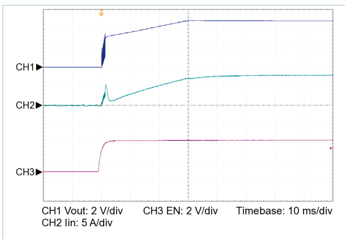
Figure 17 — Startup from EN, V_{IN} = 24\text{ V} , C_{OUT\_EXT} = 20000\ \mu\text{F} , R_{LOAD} = 0.139\ \Omega
