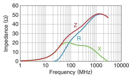
MMZ1608Y221BTD25
