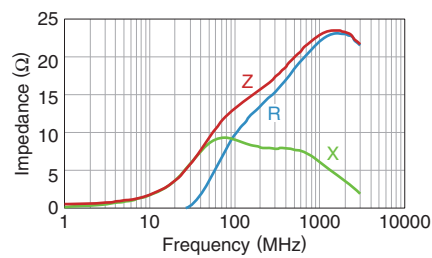
MMZ1608Y121BTD25
