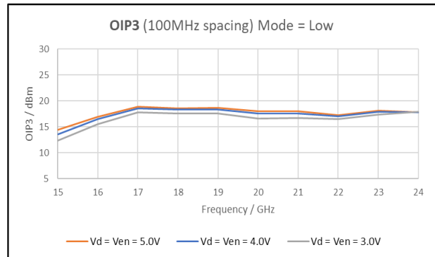
Figure 24: OIP3 100MHz spacing, P_{out} = -7\text{ dBm/tone} , low current mode
