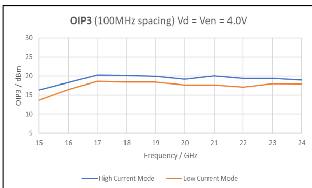
Figure 5: OIP3 100MHz spacing, P_{out} = -7dBm/ tone, V_d = V_{en} = 4.0V
