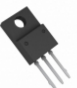
BA7820CP-E2 Rohm Semiconductor IC REG LDO 20V 1A TO220CP-3
